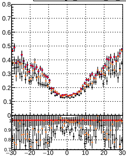
/data2/legianni/JSON-bkwd-fwd/no-modif/CMSSW_13_0_X_2023-01-24-1100/src/DQM_original DQM modified DQM modified PL DQM modified PL New1
