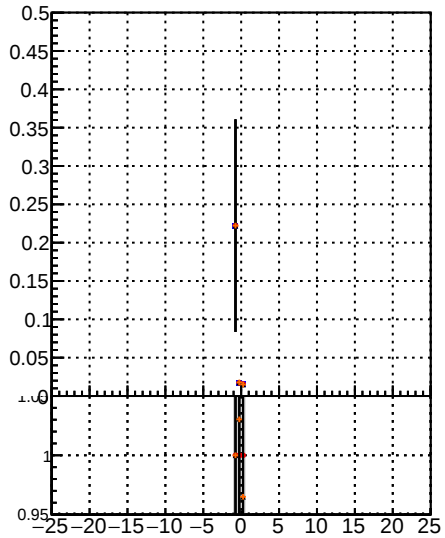
Legend: - Blue line: /data2/legion/j/JSON-bkwd-fwd/no-modif/CMSSW_13_0_X_2023-01-24-1100/src/DQM-original - Red line: BQM-modified - Orange line: BQM-modified PL New1
