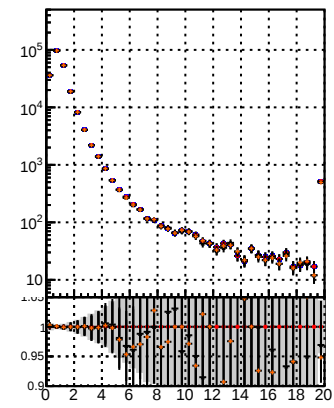
N of reco track vs. \chi^2 (data2/legion/JSON blwd fwd/no mod/CMSSW_13_0_X_2023-01-24_1100/src/BQM_original) verSet
