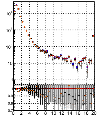
N of reco track vs. \chi^2 (data2/legions/JSON blwd fwd/no modif/CMSSW_13_0_X_2023-01-24 1400/src/DQM_original) BQM modified PL New1 BQM modified PL BQM modified PL
