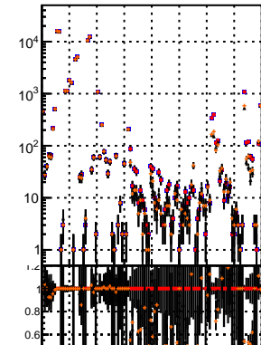
N of reco track vs. \chi^2 (data2/legions/JSON blwd fwd/no modif/CMSSW_13_0_X_2023-01-24 1400/src/DQM_original) BQM modified PL New1 BQM modified PL BQM modified PL
