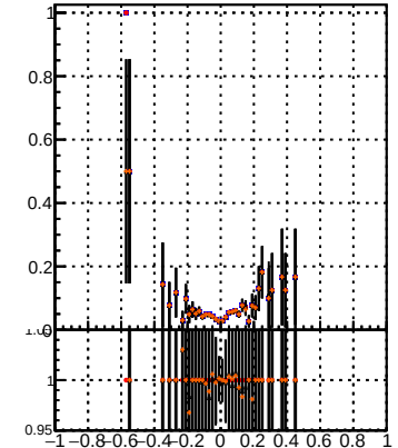
Fake rate vs dzpvp
