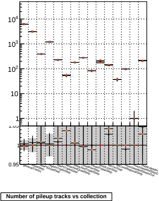
Number of pileup tracks vs collection
