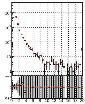
Legend: - Blue line: recoToSim JSON blwd/no-mod/GMSSW_13_0_X_2023-01-24_1100/src/DQM_original - Red line: recoToSim JSON blwd/no-mod/GMSSW_13_0_X_2023-01-24_1100/src/DQM_modified - Orange line: recoToSim JSON blwd/no-mod/GMSSW_13_0_X_2023-01-24_1100/src/DQM_New1
