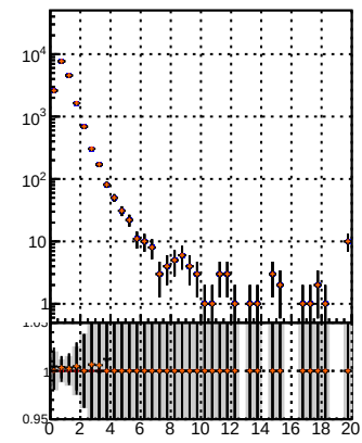
N of reco track vs. \chi^2 (data2/legion/JSON blwd fwd/no mod/GMSSW_13_0_X_2023-01-24_1100/src/DQM_original) BSM modified PL New1
