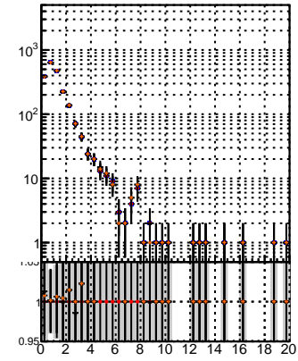
N of reco track vs. \chi^2 (data2/legion/JSON blwd fwd/no modif/CMSSW_13_0_X_2023-01-24 1400/src/DQM_original)
