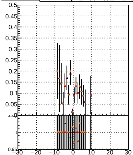
Fake rate vs v DQM modified PL New1
