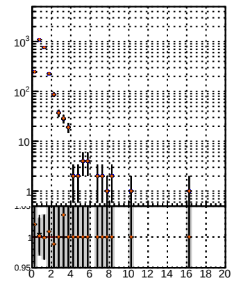
N of reco track vs. \chi^2 (data2) lognormal JSON blwd fwd no modif CMSSW_13_0_X_2023-01-24_1100/src/BQM_original BSM modified PL New1
