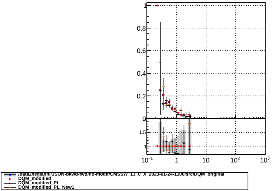
fake+duplicates vs p_T
