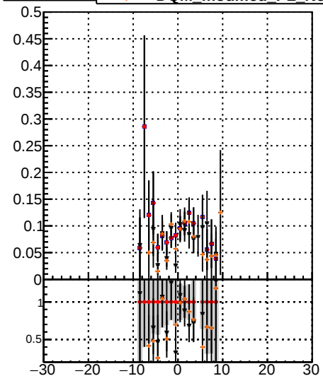
Fake rate vs vertpos Legend: data2/legianni/JSON-bkwd-fwd/no-modif/CMSSW_13_0_X_2023-01-24-1100/src/DQM_original DQM modified PL DQM modified PL New1
