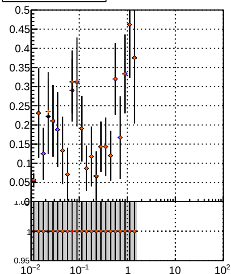
Fake rate vs vertpos Legend: - DQM modified PL - DQM modified PL New1
