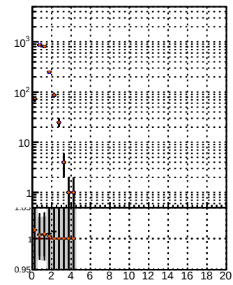
N of reco track vs. (data2/legion/JSON/blwd-fwd-no-mod/GMSSW_13_0_X_2023-01-24_1100/src/BQM_original
