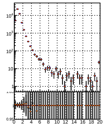
N of reco track vs. \chi^2 (data2/legion/JSON/blwd-fwd/no-modif/GMSSW_13_0_X_2023-01-24_1100/src/DQM_original BSW modified PL New1
