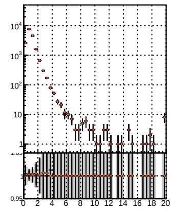
N of reco track vs. \chi^2 for BSW modified PL New1
