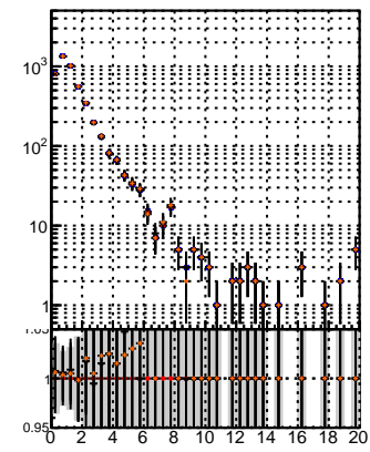
N of reco track vs. \chi^2 (data2/legion/JSON blwd fwd/no mod/CMSW_13_0_X_2023 01 24 1400/src/DQM_original)
