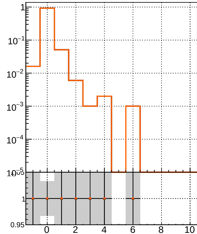
TruePVLocationIndexInRecoVertexCollection
