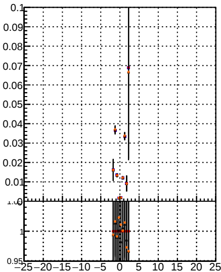
Fake rate vs dxy Legend: ■ /data2/legion/JSON-bkwd-fwd/no-modif/CMSSW_13_0_X_2023-01-24-1100/src/DQM_original ■ DQM_modified_PL ■ DQM_modified_PL_New1
