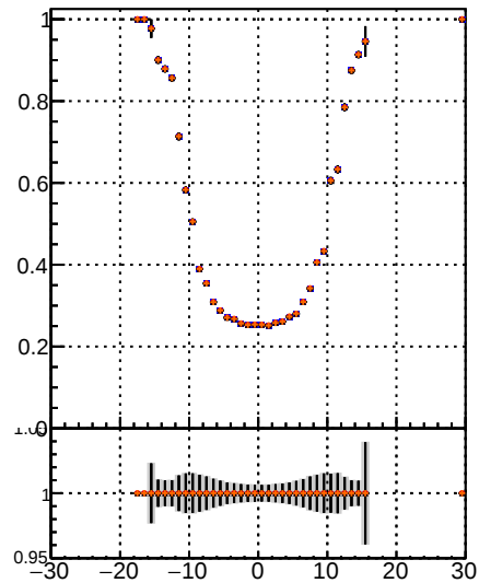
Fake rate vs d /data2/legion/JSON-bkwd-fwd/no-modif/CMSSW_13_0_X_2023-01-24-1100/src/DQM_original DQM modified PL New1
