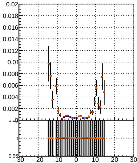
Fake rate vs d /data2/legion/JSON-bkwd-fwd/no-modif/CMSSW_13_0_X_2023-01-24-1100/src/DQM_original DQM modified PL New1
