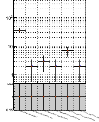
N of associated (recoToSim) loopier tracks vs. \chi^2
