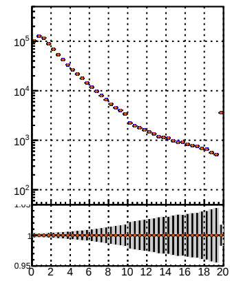
N of reco track vs. \chi^2 (data2/legion/JSON-blwd-fwd/no-modif/GMSSW_13_0_X_2023-01-24_1100/src/BQM_original) verSet
