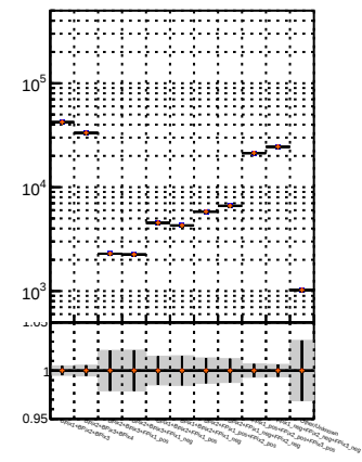
N of reco track vs. \chi^2 (data2/legion/JSON-blwd-fwd/no-modif/GMSSW_13_0_X_2023-01-24_1100/src/BQM_original) verSet
