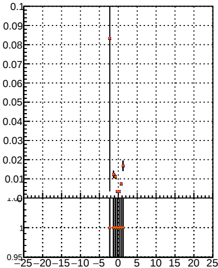
Legend: - Blue line: /data2/legion/JSON-bkwd-fwd/no-modif/CMSSW_13_0_X_2023-01-24-1100/src/DQM_original - Red line: BQM modified PL New1 - Black line: BQM modified PL New1
