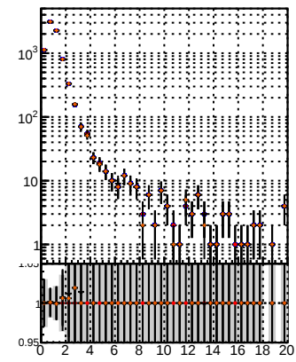
N of reco track vs. \chi^2 (data2/legion/JSON/blwd-fwd/no-mod/CMSW_13_0_X_2023-01-24_1100/src/DQM_original)
