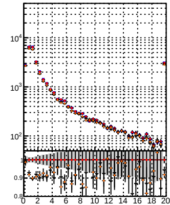
N of reco track vs. \chi^2 (data2/region1/JSON/blwd-fwd/no-mod/GMSSW_13_0_X_2023_01_24_1100/src/BQM_original)
