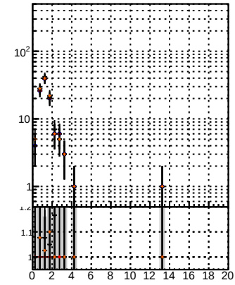
N of reco track vs. \chi^2 (data?/origin//JSON blwd fwd no modif/GMSSW_13_0_X_2023-01-24_1100/src/DQM_original)
