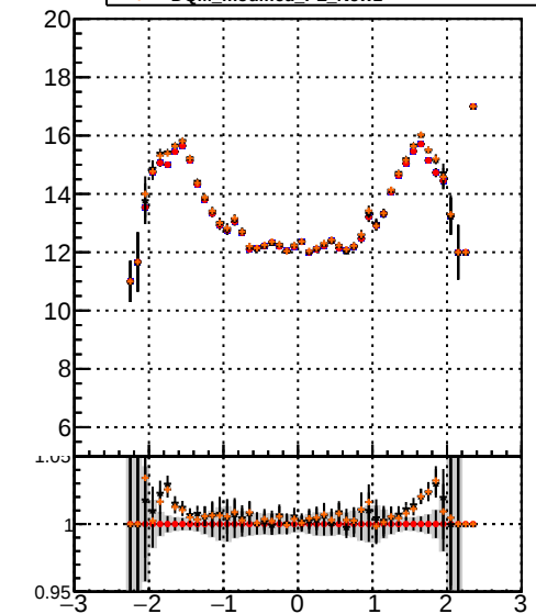
mean hit Legend: /data2/legianni/JSON-bkwd-fwd/no-modif/CMSSW_13_0_X_2023-01-24-1100/src/DQM_original (blue line), DQM_modified (red line), DQM_modified_PL (black line), DQM_modified_PL_New1 (orange line)
