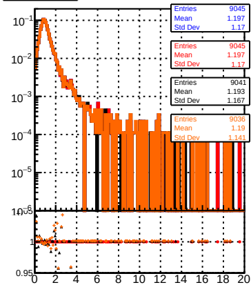
normalized \chi^2
