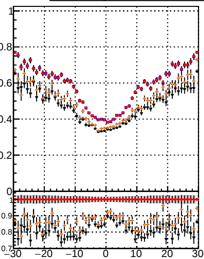
[Legend: DQM modified PL, DQM modified PL New1, DQM modified PL] Fake rate vs vertpos
