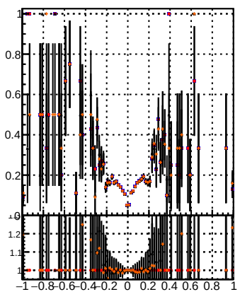
/data2/legiannn/JSON-bkwd-fwd/no-modif/CMSSW_13_0_X_2023-01-24-1100/src/DQM_original DQM_modified DQM_modified_PL DQM_modified_PL_New1
