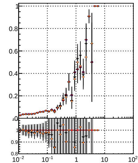
/data2/legianni/JSON-bkwd-fwd/no-modif/CMSSW_13_0_X_2023-01-24-1100/src/DQM_original Fake rate vs v DQM modified PL DQM modified PL New1
