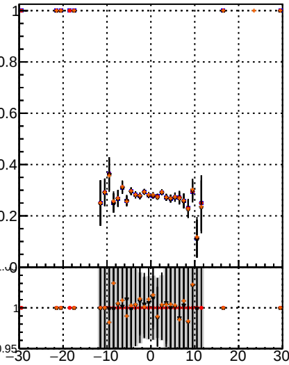
Fake rate vs vertpos data2/legianni/JSON-bkwd-fwd/no-modif/CMSSW_13_0_X_2023-01-24-1100/src/DQM_original DQM modified PL New1
