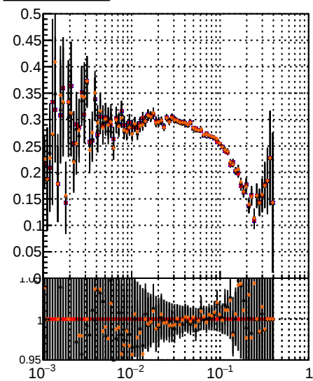
Fake rate vs dr Legend: - data2/legianni/JSON-bkwd-fwd/no-modif/CMSSW_13_0_X_2023-01-24-1100/src/DQM_original - DQM modified PL New1 - DQM modified PL New1
