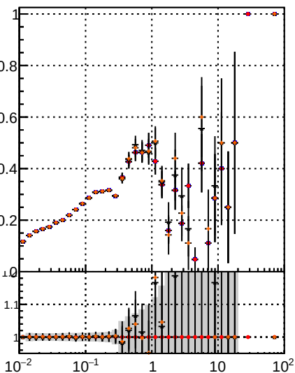
/data2/legianni/JSON-bkwd-fwd/no-modif/CMSSW_13_0_X_2023-01-24-1100/src/DQM_original Fake rate vs v DQM modified PL New1 DQM modified PL New1
