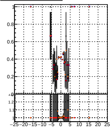
Efficiency /data2/legianni/JSON-bkwd-fwd/no-modif/CMSSW_13_0_X_2023-01-24-1100/src/DQM_original DQM_modified DQM_modified_PL DQM_modified_PL_New1
