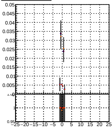
Efficiency /data2/legianni/JSON-bkwd-fwd/no-modif/CMSSW_13_0_X_2023-01-24-1100/src/DQM_original DQM_modified DQM_modified_PL DQM_modified_PL_New1
