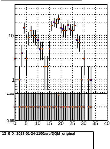
N of associated tracks (simToReco) vs hit
