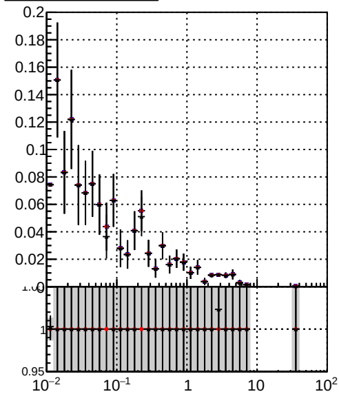
Efficiency vs vertpos Legend: — /data2/legianni/JSON-bkwd-fwd/no-modif/CMSSW_13_0_X_2023-01-24-1100/src/DQM_original — DQM_modified — DQM_modified_PL
