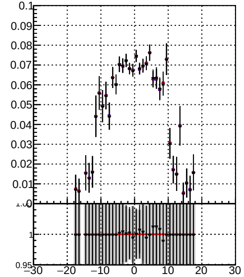
Efficiency vs vertpos Legend: — /data2/legianni/JSON-bkwd-fwd/no-modif/CMSSW_13_0_X_2023-01-24-1100/src/DQM_original — DQM_modified — DQM_modified_PL
