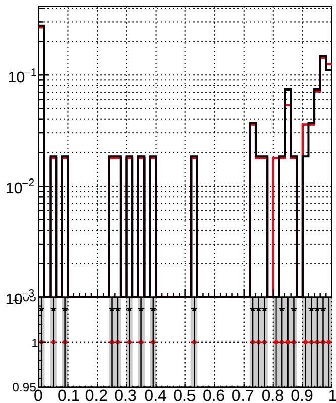
RecoPVAssoc2GenPVNotMatched_Purity
