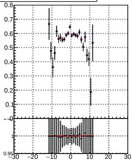
/data2/legianni/JSON-bkwd-fwd/no-modif/CMSSW_13_0_X_2023-01-24-1100/src/DQM_original DQM_modified DQM_modified_PL Fake rate vs v
