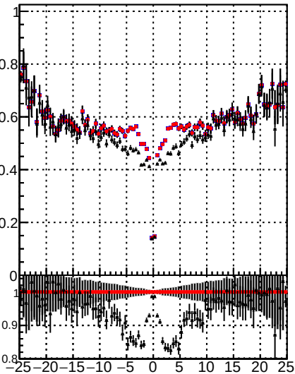
/data2/legianni/JSON-bkwd-fwd/no-modif/CMSSW_13_6_X_2023-01-24-1100/src/DQM_original Fake rate vs d
