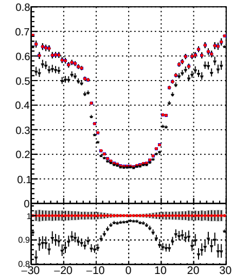
/data2/legianni/JSON-bkwd-fwd/no-modif/CMSSW_13_6_X_2023-01-24-1100/src/DQM_original Fake rate vs d
