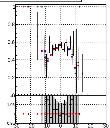
Fake rate vs vertpos Legend: \blacksquare /data2/legianni/JSON-bkwd-fwd/no-modif/CMSSW_13_0_X_2023-01-24-1100/src/DQM_original \bullet DQM_modified \star DQM_modified_PL
