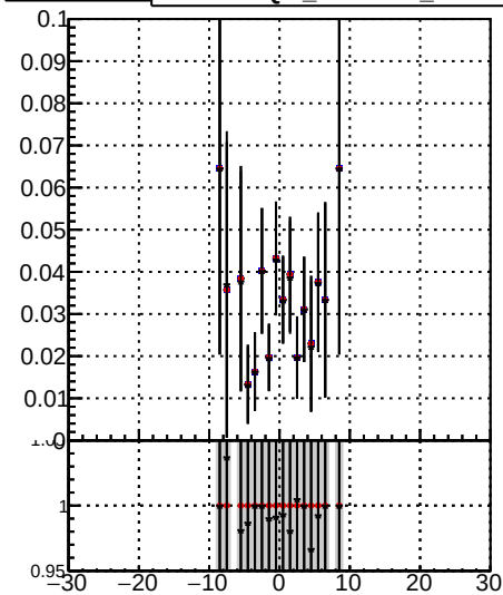
/data2/legianni/JSON-bkwd-fwd/no-modif/CMSSW_13_0_X_2023-01-24-1100/src/DQM_original DQM_modified DQM_modified_PL Fake rate vs v
