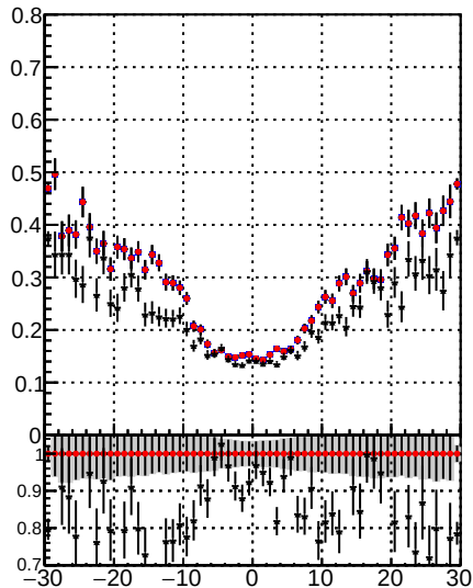
— /data2/legianni/JSON-bkwd-fwd/no-modif/CMSSW_13_0_X_2023-01-24-1100/src/DQM_original — BQM_modified_PL
