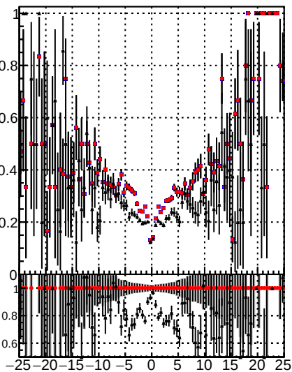
— /data2/legianni/JSON-bkwd-fwd/no-modif/CMSSW_13_0_X_2023-01-24-1100/src/DQM_original — BQM_modified_PL
