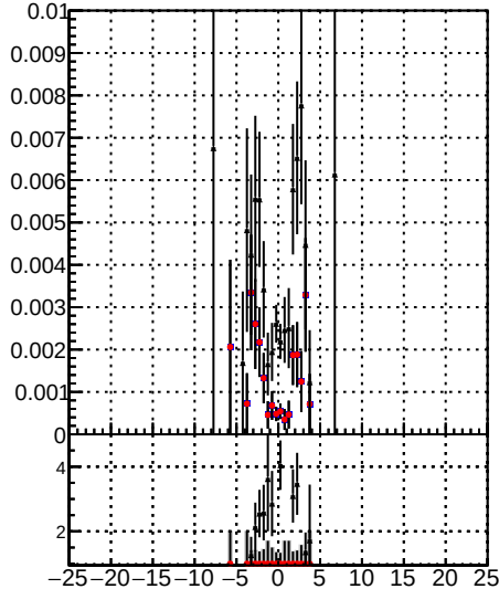
— /data2/legianni/JSON-bkwd-fwd/no-modif/CMSSW_13_0_X_2023-01-24-1100/src/DQM_original — BQM_modified_PL
