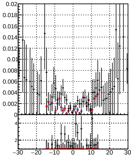
— /data2/legianni/JSON-bkwd-fwd/no-modif/CMSSW_13_0_X_2023-01-24-1100/src/DQM_original — BQM_modified_PL
