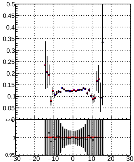
Legend: - Blue line: /data2/legianni/JSON-bkwd-fwd/no-modif/CMSSW_13_0_X_2023-01-24-1100/src/DQM_original - Red line: BQM modified PL
