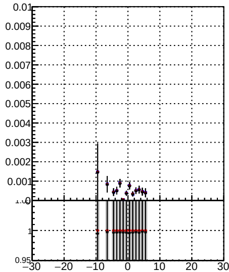
Legend: - Blue line: /data2/legianni/JSON-bkwd-fwd/no-modif/CMSSW_13_0_X_2023-01-24-1100/src/DQM_original - Red line: BQM modified PL
