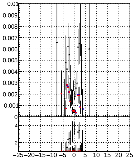
Legend: - /data2/legianni/JSON-bkwd-fwd/no-modif/CMSSW_13_0_X_2023-01-24-1100/src/DQM\_original (black line with error bars) - BCM\_modified\_PL (red line with error bars)
