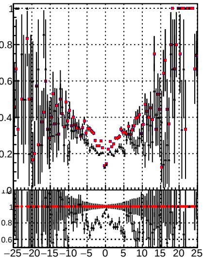
Legend: - /data2/legianni/JSON-bkwd-fwd/no-modif/CMSSW_13_0_X_2023-01-24-1100/src/DQM\_original (black line with error bars) - BCM\_modified\_PL (red line with error bars)
