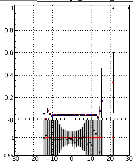
Legend for all plots: ● /data2/legianni/JSON-bkwd-fwd/no-modif/CMSSW_13_0_X_2023-01-24-1100/src/DQM_original ● DQM_modified ● DQM_modified_PL
