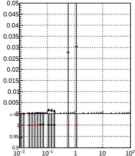
Legend for all plots: ● /data2/legianni/JSON-bkwd-fwd/no-modif/CMSSW_13_0_X_2023-01-24-1100/src/DQM_original ● DQM_modified ● DQM_modified_PL
