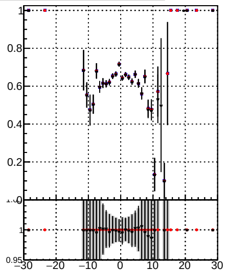
/data2/legianni/JSON-bkwd-fwd/no-modif/CMSSW_13_0_X_2023-01-24-1100/src/DQM_original Fake rate vs verpos DQM_modified DQM_modified_PL
