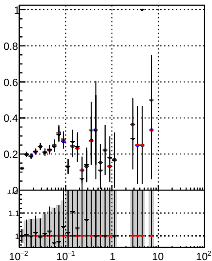
/data2/legianni/JSON-bkwd-fwd/no-modif/CMSSW_13_0_X_2023-01-24-1100/src/DQM_original Fake rate vs verpos DQM_modified DQM_modified_PL
