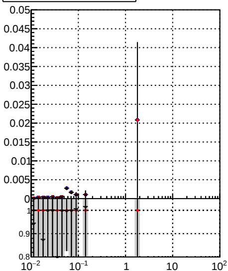
Legend: ■ /data2/legianni/JSON-bkwd-fwd/no-modif/CMSSW_13_0_X_2023-01-24-1100/src/DQM_original ● DQM_modified + DQM_modified_PL
