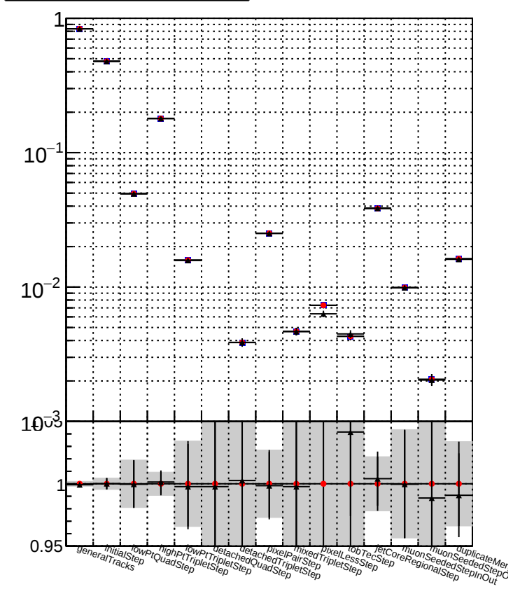
Duplicates rate vs collection Legend: /data2/legianni/JSON-bkwd-fwd/no-modif/CMSSW_13_0_X_2023-01-24-1100/src/DQM_original DQM_modified DQM_modified_PL
